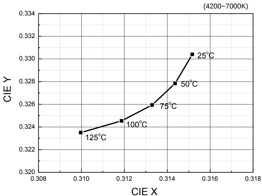
Fig 8. Chromaticity Coordinate vs. Junction Temperature, I_F=40\text{mA}
